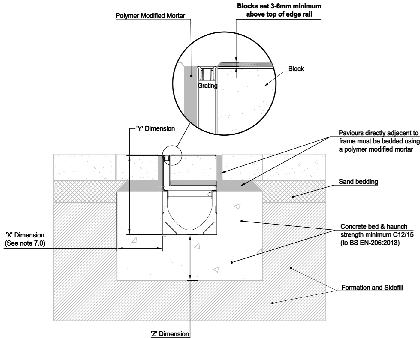
1 : 5 ACO RainDrain Brickslot B 125 Access Cover Block Pavement (Option 1 and 2)
