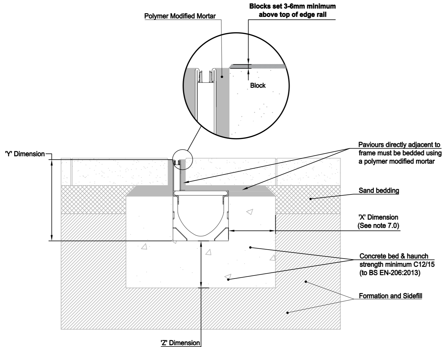
1 : 5 ACO RainDrain Brickslot B 125 Block Pavement (Option 1 and 2)
