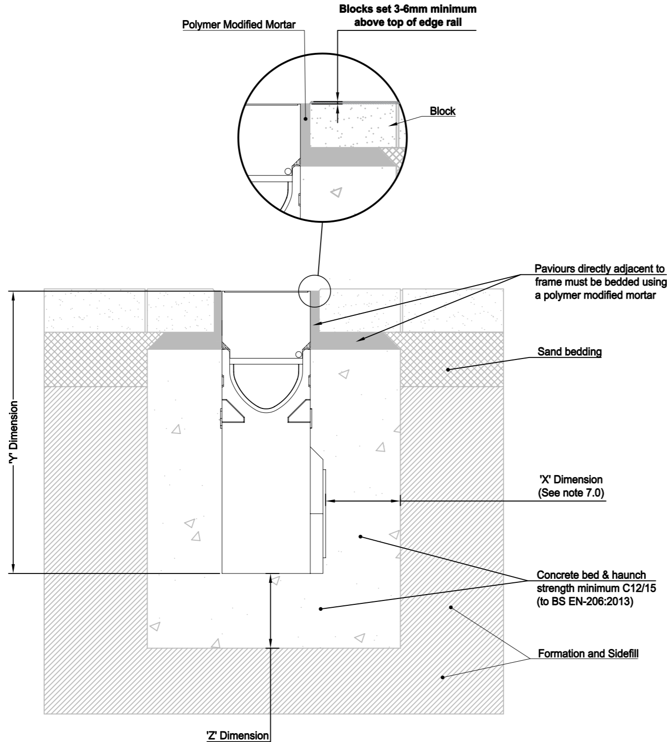
1 : 5 ACO RainDrain Brickslot B125 Sump Access Cover Block Pavement (Option 1 and 2)
